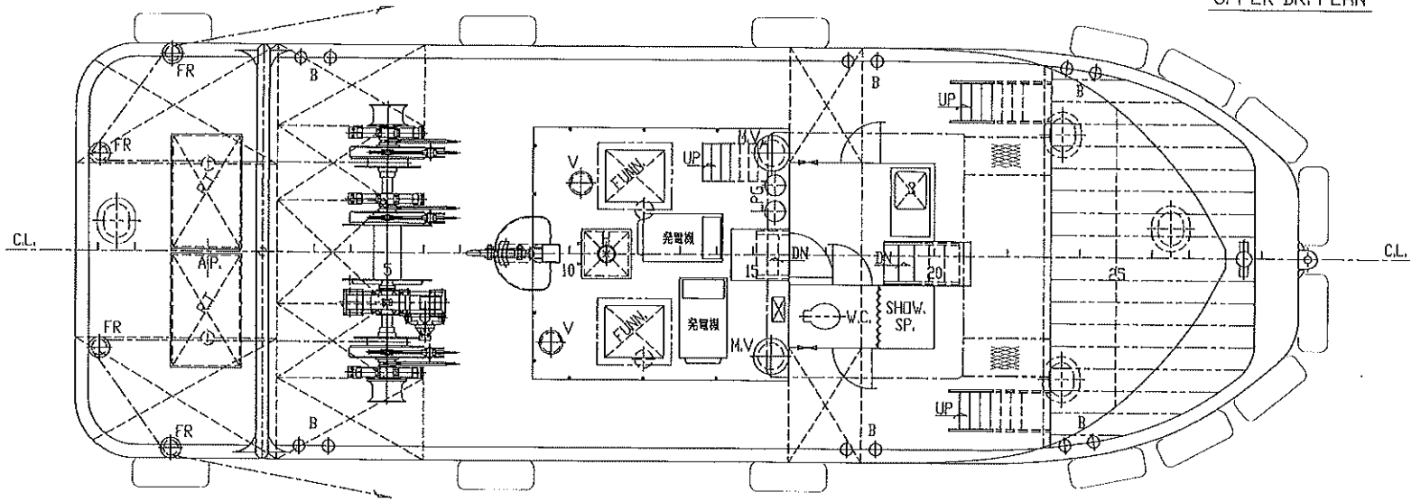
UPPER DK. PLAN
