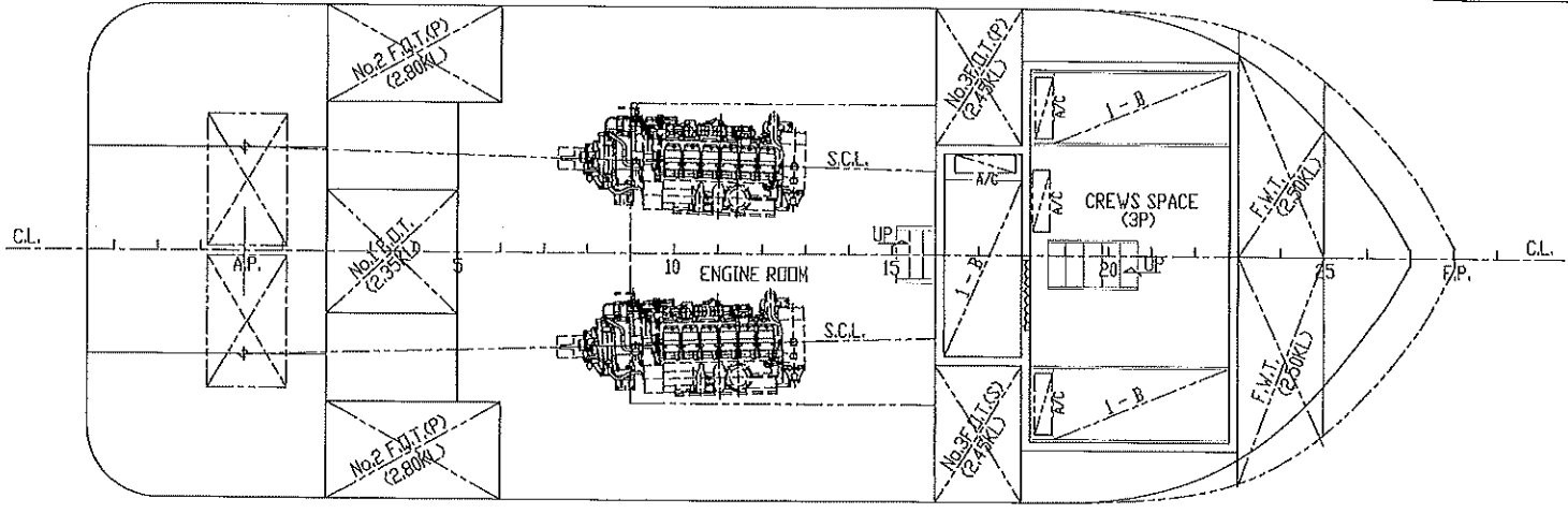
BOTTOM PLAN
