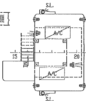
2ND. DECK (D.H. = 1350)
