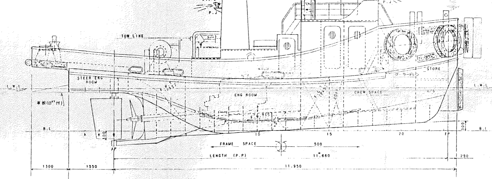
DECK PLAN
