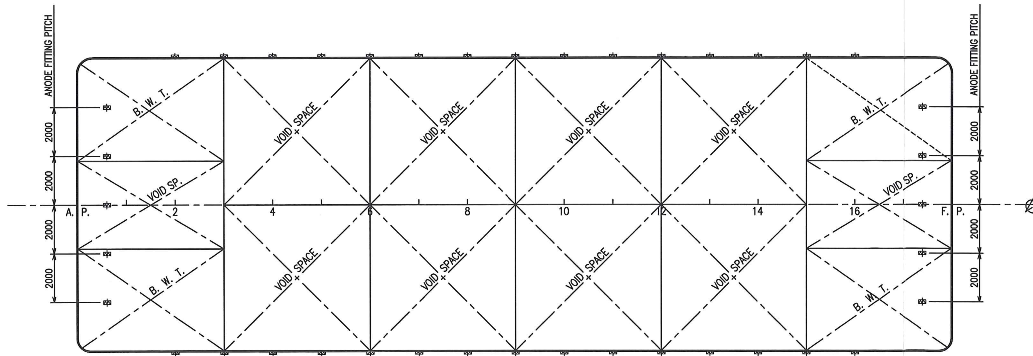
DECK PLAN
